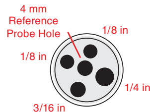
Multi-hole type 4 (ITC-155)
