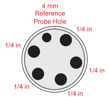
Multi-hole type 5 (ITC-320/650)
