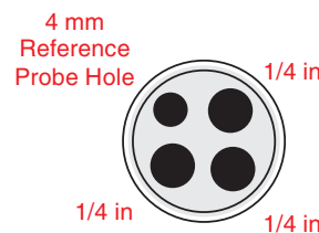
Multi-hole type 5 (ITC-155)
