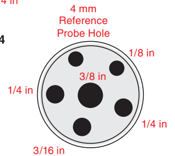
Multi-hole type 6 (ITC-320/650)
